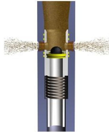
Open Position FLOW THRU PORT
